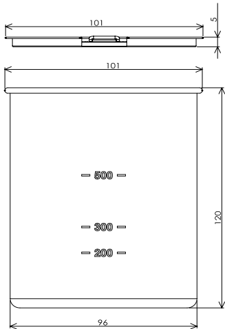
Cozy Bag 750 / Weight: 40 g
