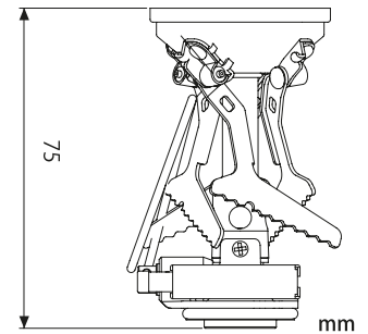
Amicus w/Stealth Igniter 81g w/o igniter 75g
