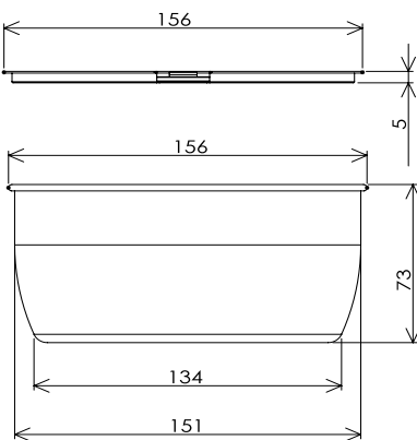
Cozy Bag 1100 / Weight: 46 g
